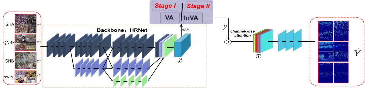
Figure 3: The pipeline of the proposed DKPNet. It contains two-stage training: VA and InVA are used in Stage-I and Stage-II, respectively. Before Stage-II training, we will first get the CL labels from the attention outputs of VA by clustering, and then reassign the training images with these CL labels.
