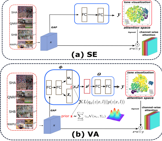
Figure 2: Comparisons between SE and VA. Different datasets are trained jointly. \odot means channel-wise product. One can observe that SE attention outputs are confusing, while our VA can produce more separable attention distributions for different domains by introducing the Gaussian Mixture distributed latent variable z .
